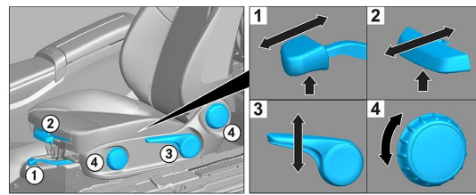
Aggustament tas-sit (b'mod mekkaniku)
