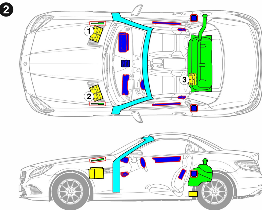
② On-board electrical system battery, right-hand drive
